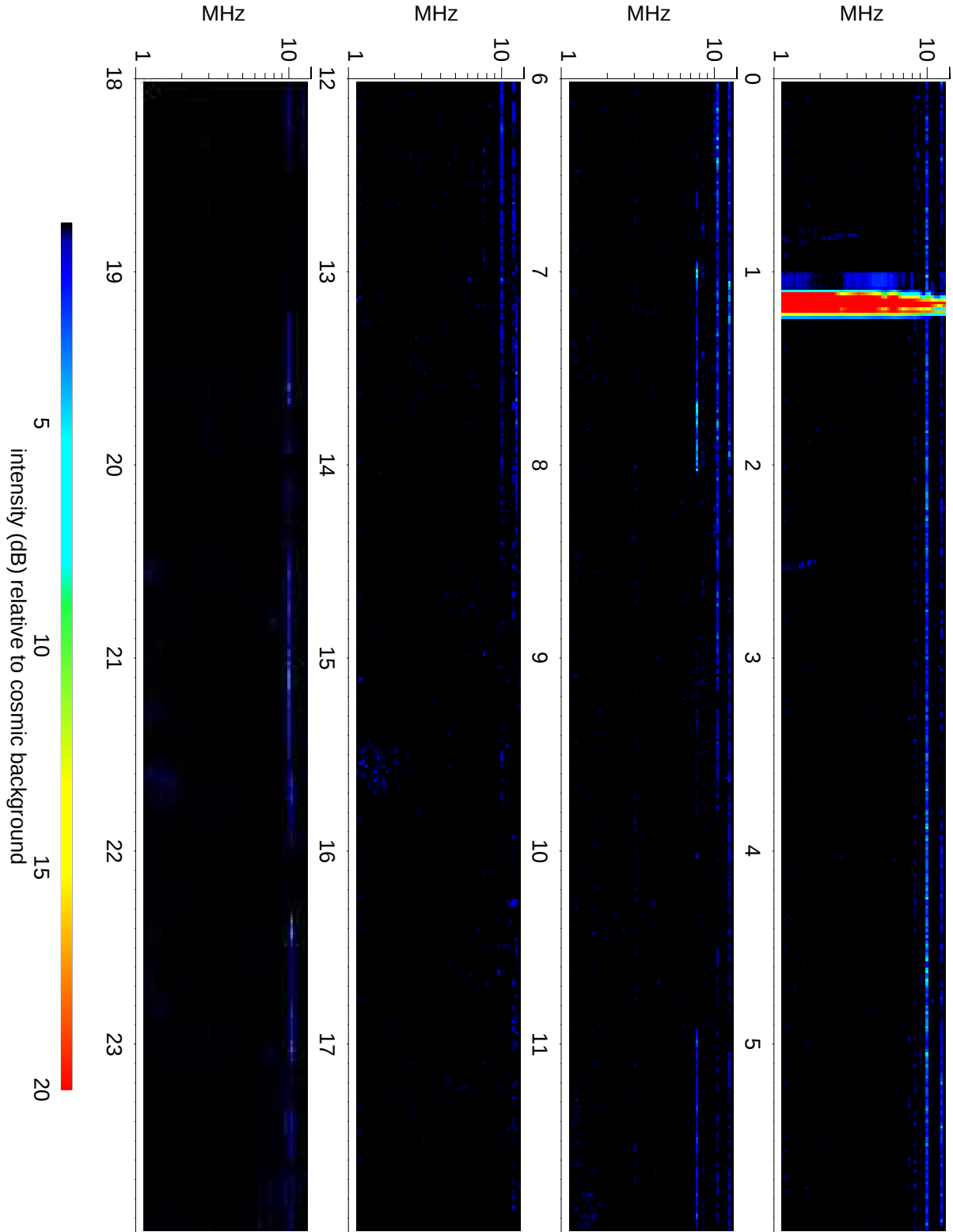
Wind Waves RAD2 receiver: 2018/05/16
