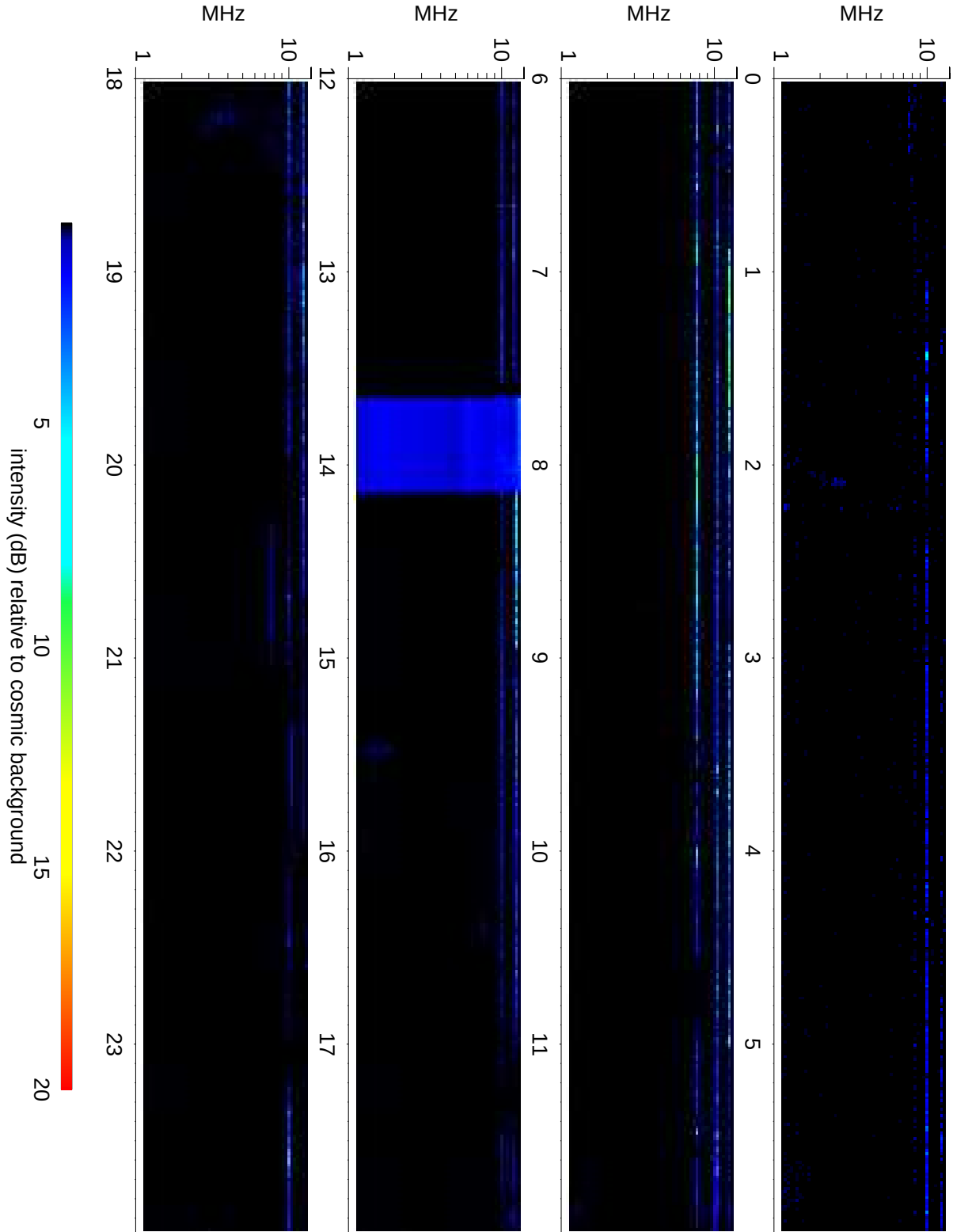
Wind Waves RAD2 receiver: 2018/07/22
