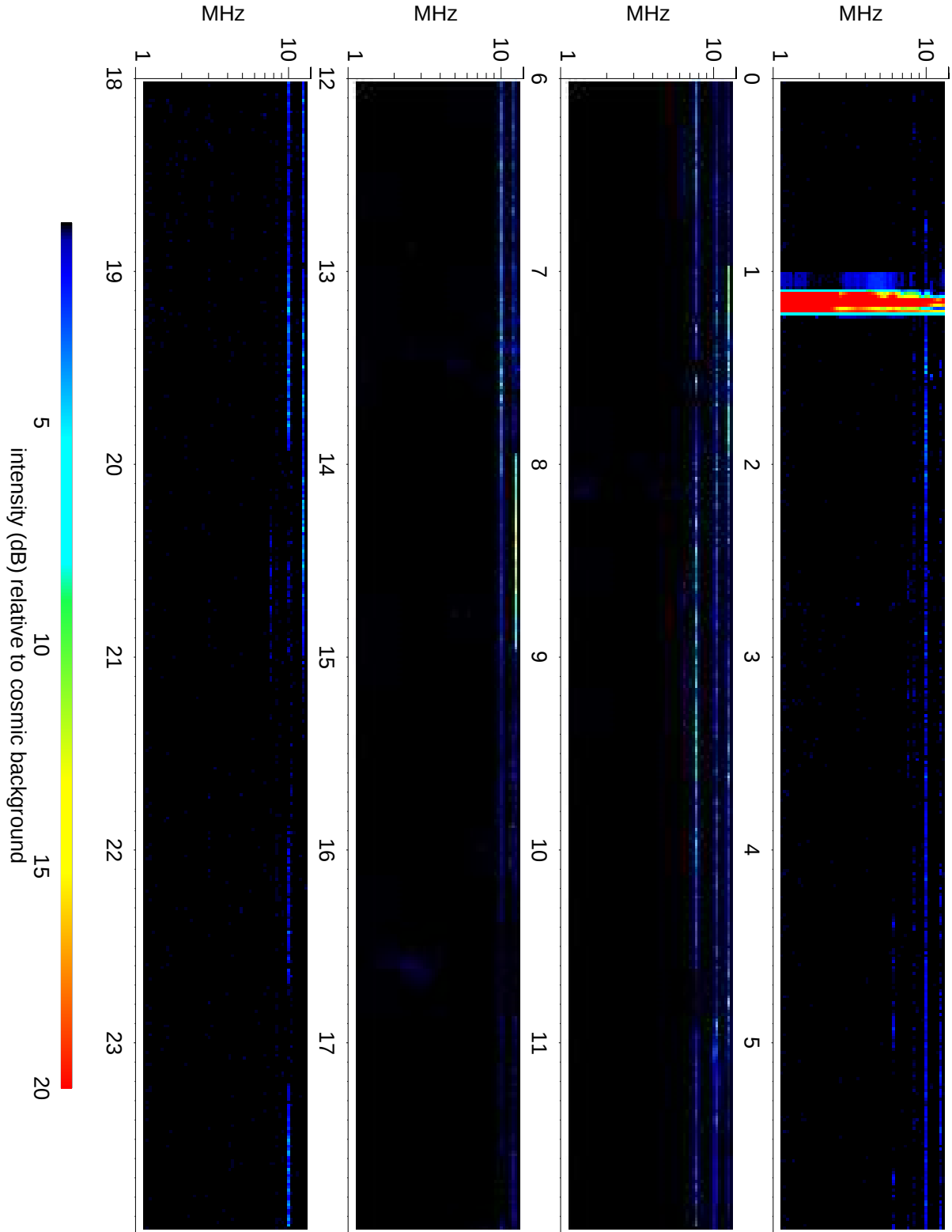
Wind Waves RAD2 receiver: 2018/07/25
