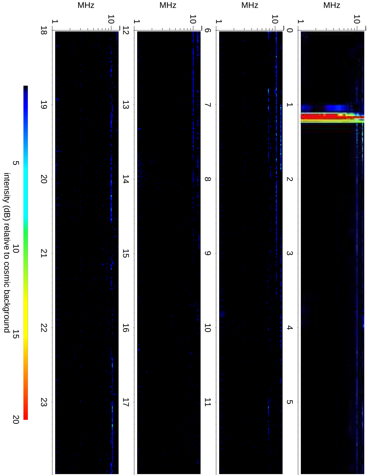
Wind Waves RAD2 receiver: 2018/09/13
