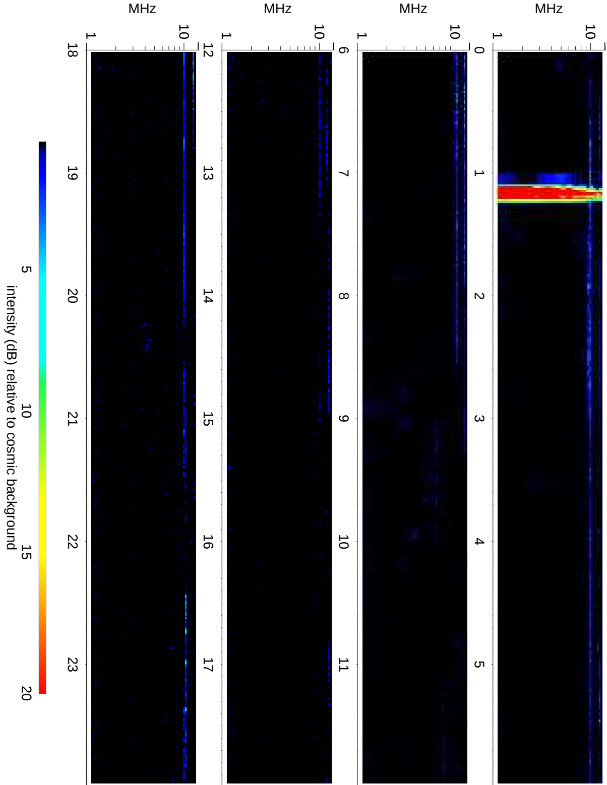
Wind Waves RAD2 receiver: 2018/09/23
