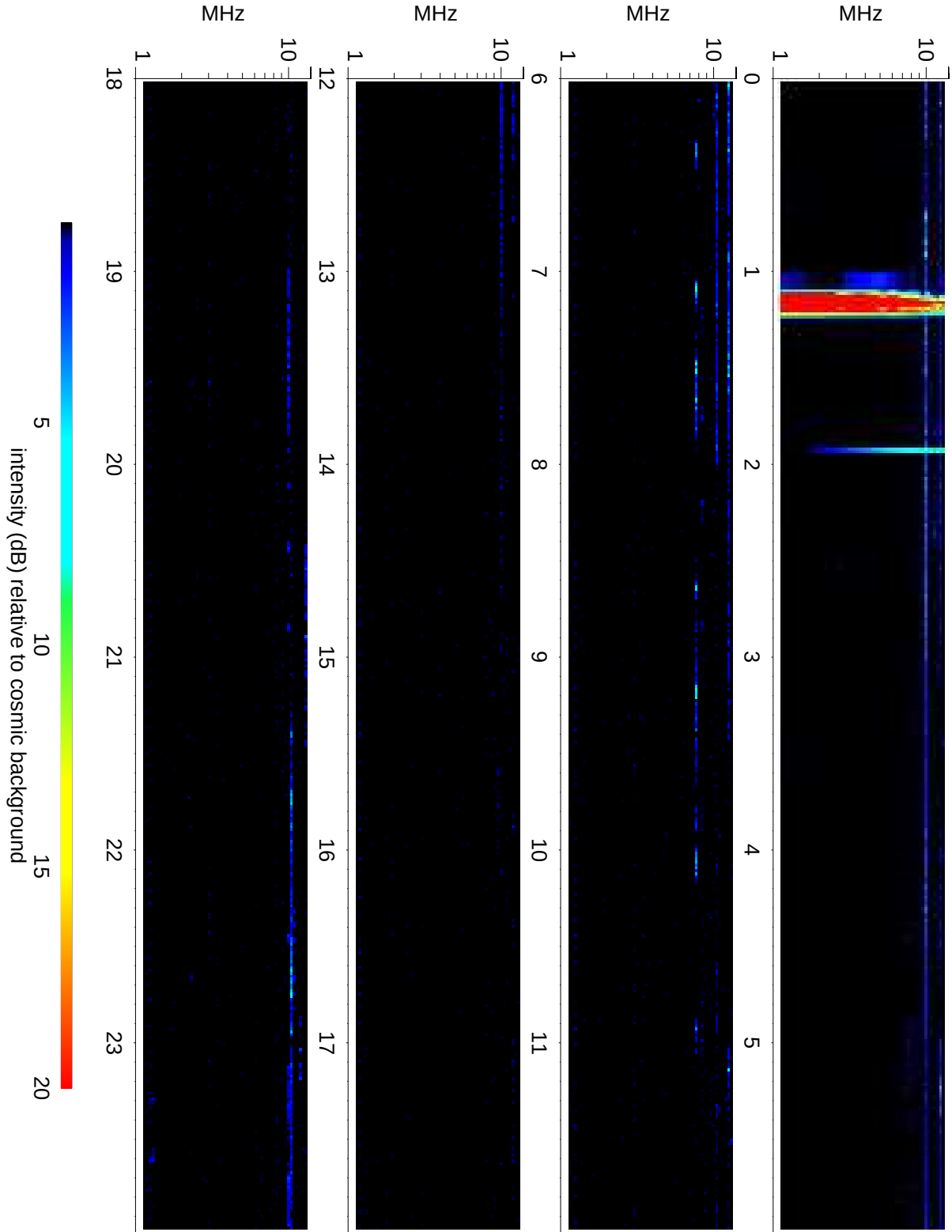
Wind Waves RAD2 receiver: 2018/10/01
