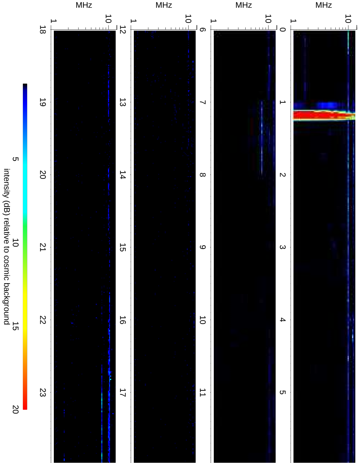
Wind Waves RAD2 receiver: 2018/10/19
