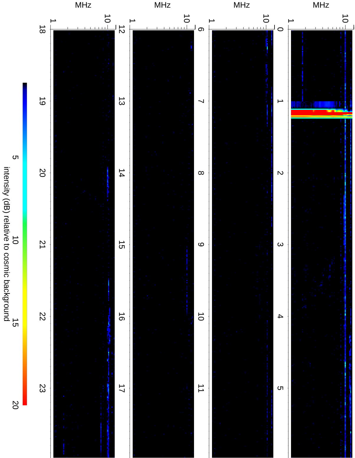
Wind Waves RAD2 receiver: 2018/10/21
