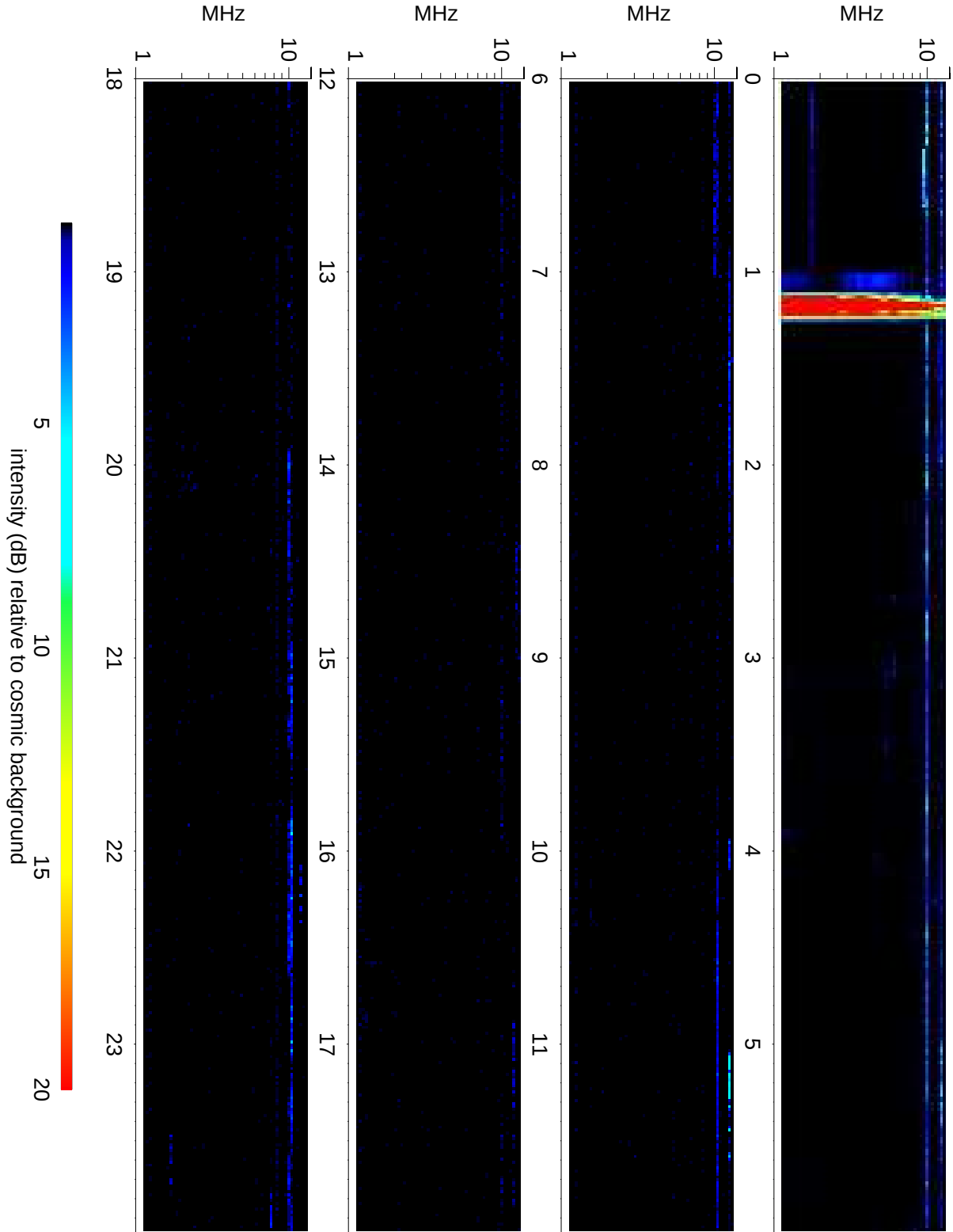
Wind Waves RAD2 receiver: 2018/10/27
