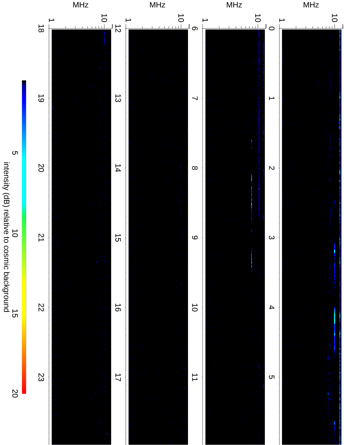
Wind Waves RAD2 receiver: 2018/11/19
