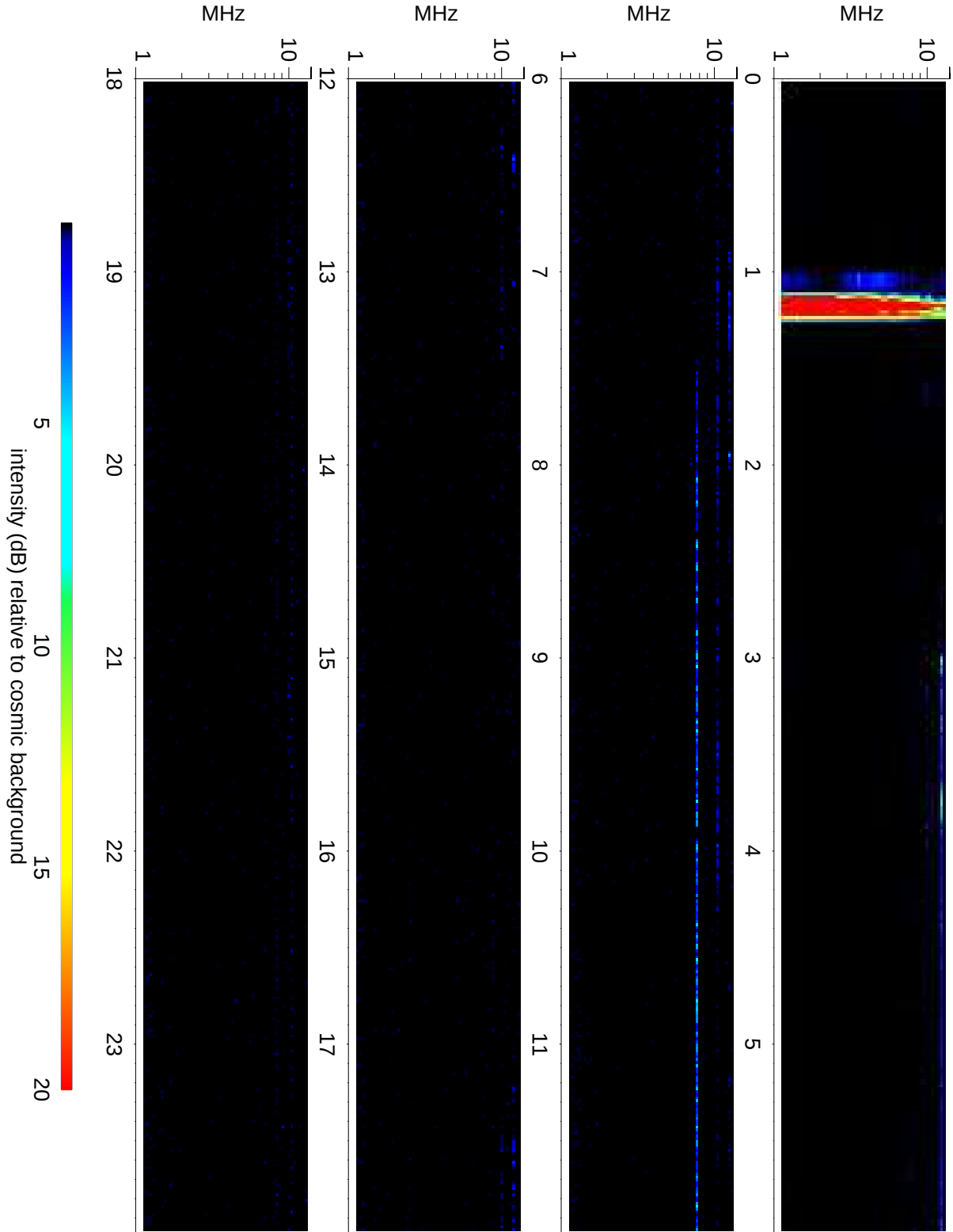
Wind Waves RAD2 receiver: 2018/12/04
