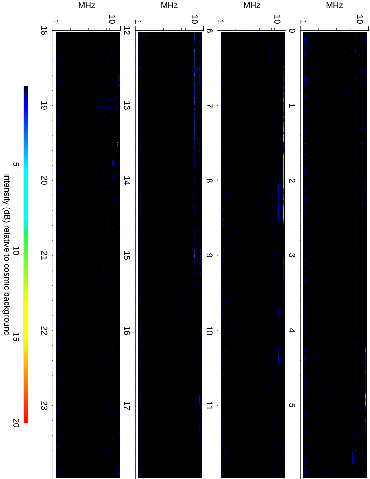
Wind Waves RAD2 receiver: 2018/12/15
