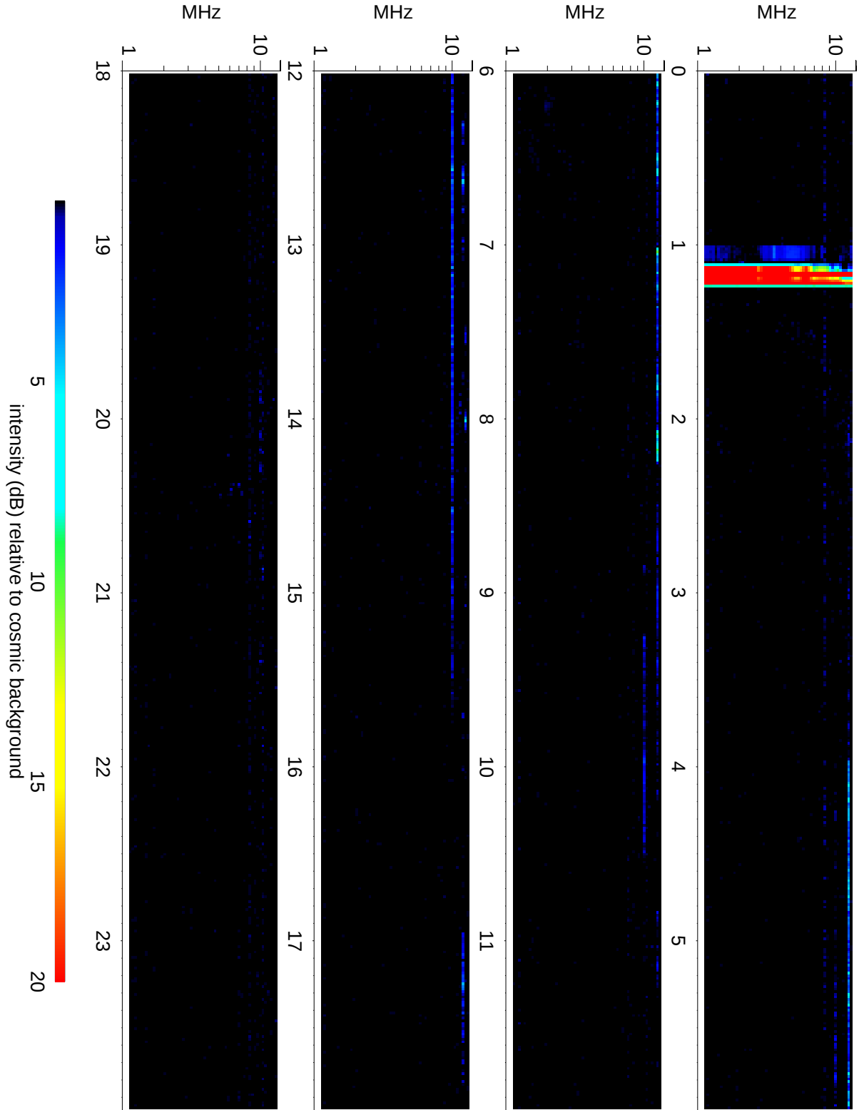
Wind Waves RAD2 receiver: 2018/12/22
