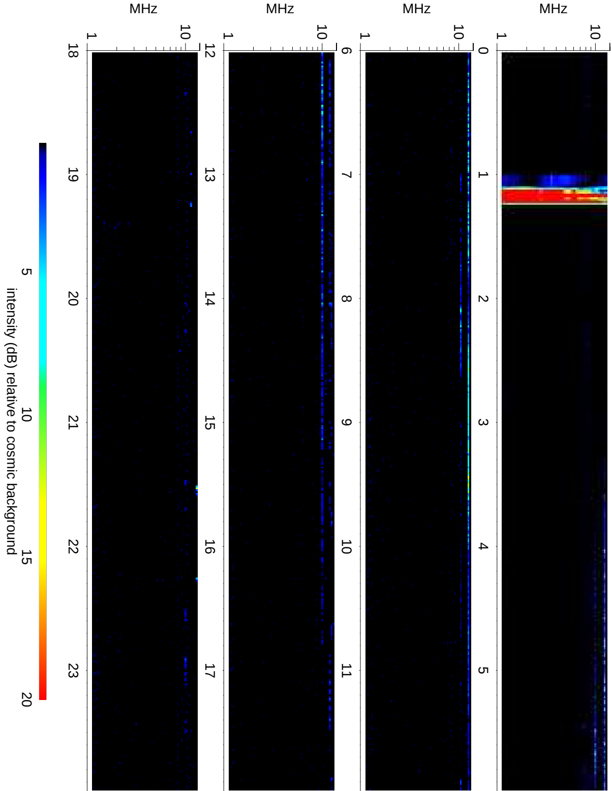
Wind Waves RAD2 receiver: 2018/12/30
