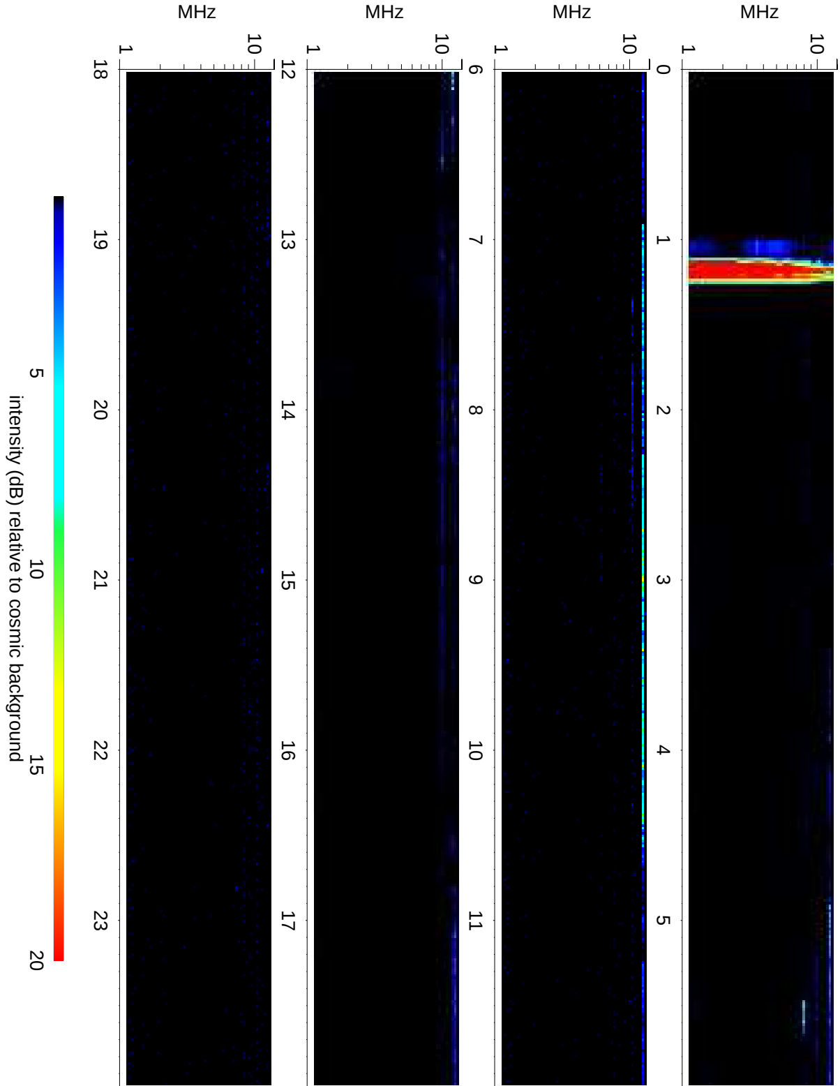
Wind Waves RAD2 receiver: 2020/01/06
