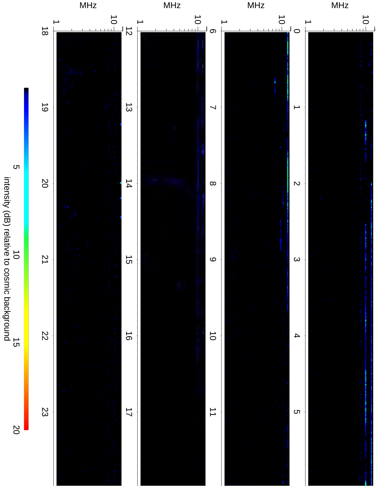
Wind Waves RAD2 receiver: 2020/02/10
