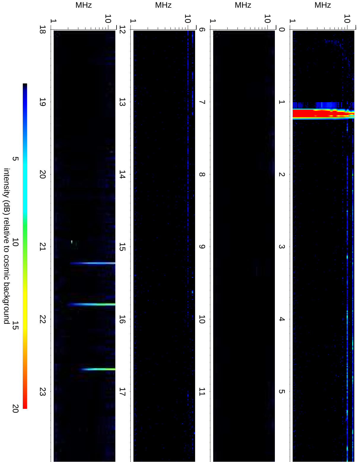
Wind Waves RAD2 receiver: 2020/02/11
