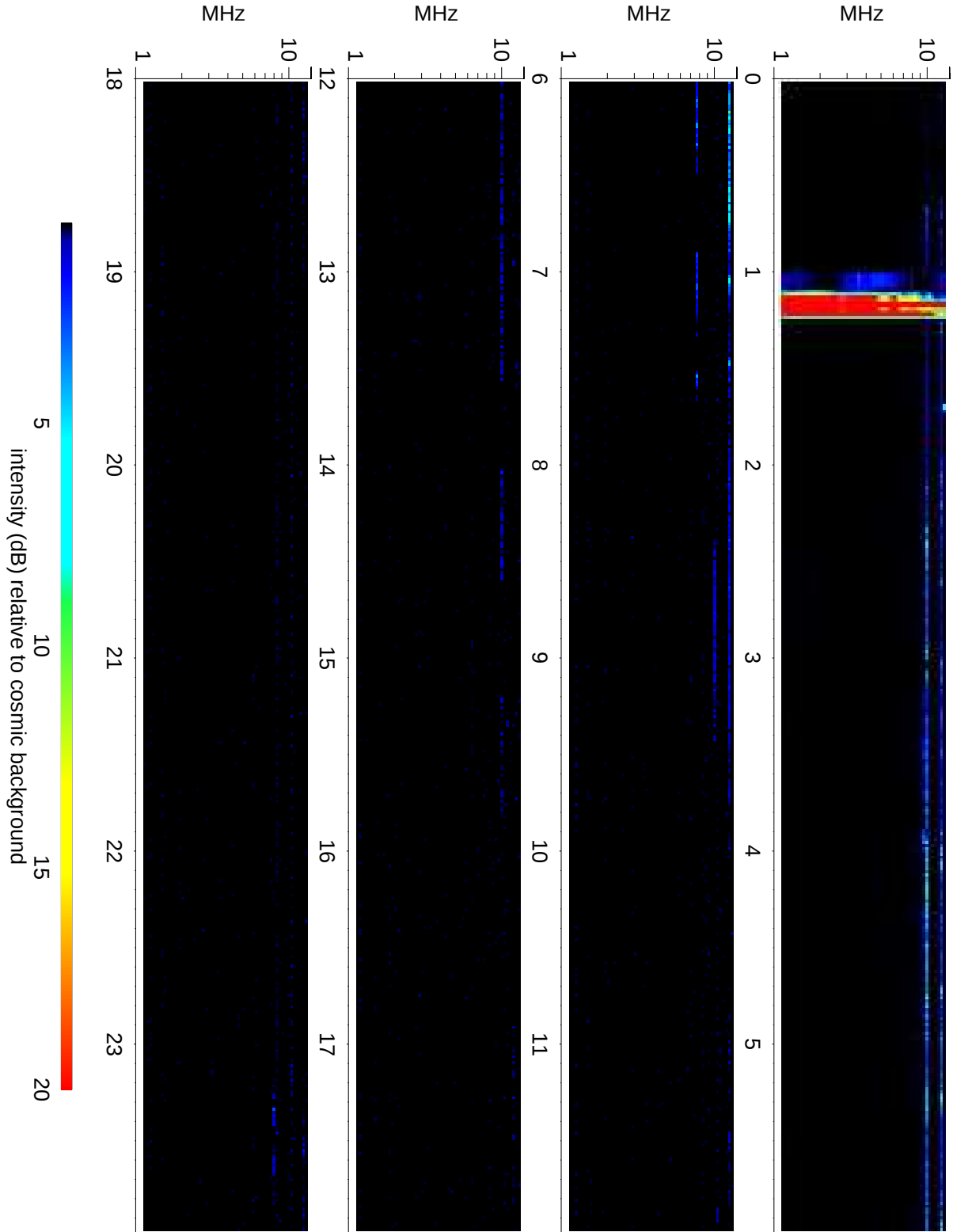
Wind Waves RAD2 receiver: 2020/02/17
