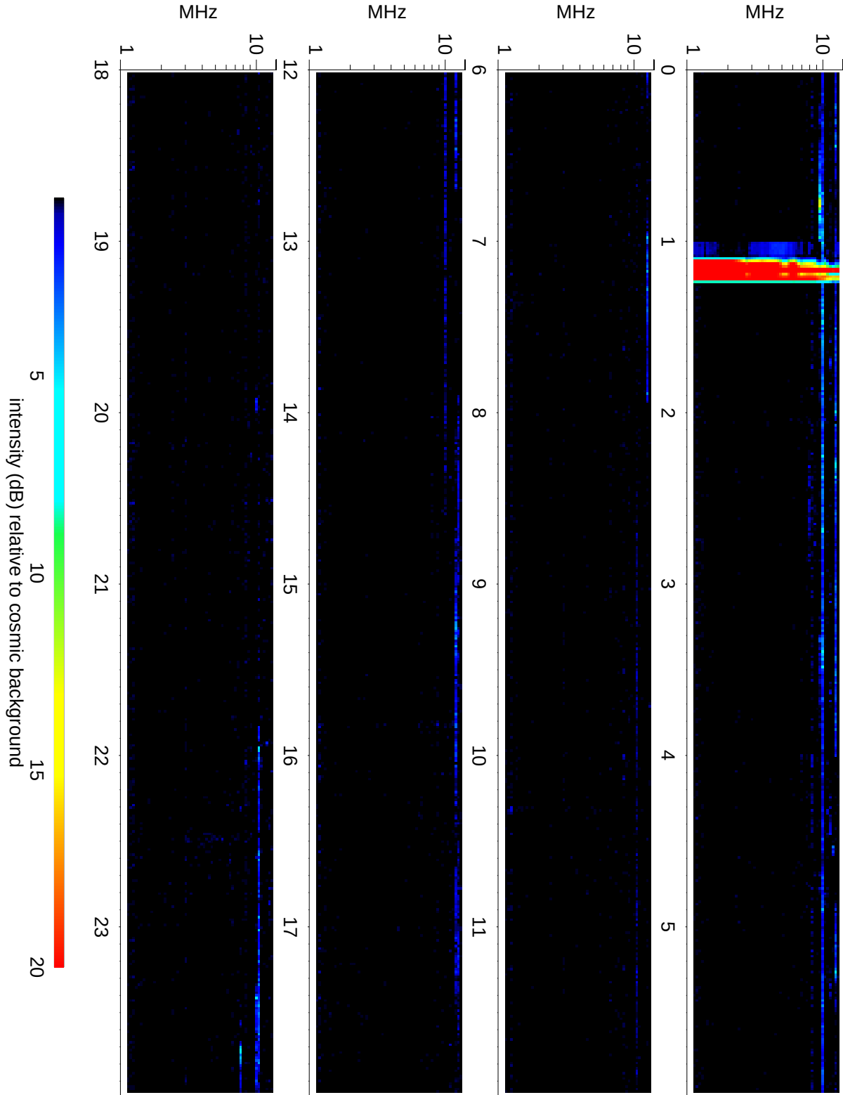
Wind Waves RAD2 receiver: 2020/04/11
