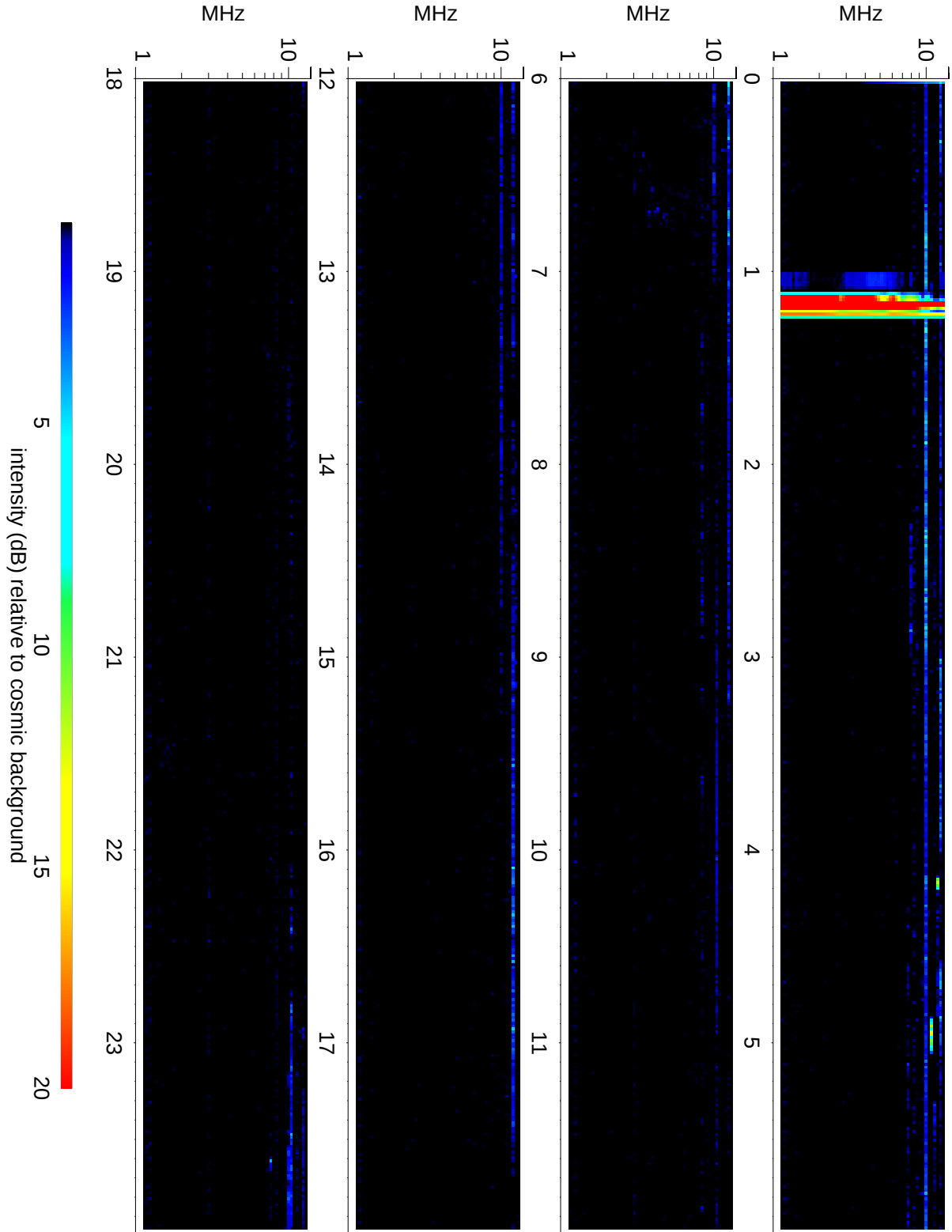
Wind Waves RAD2 receiver: 2020/04/17
