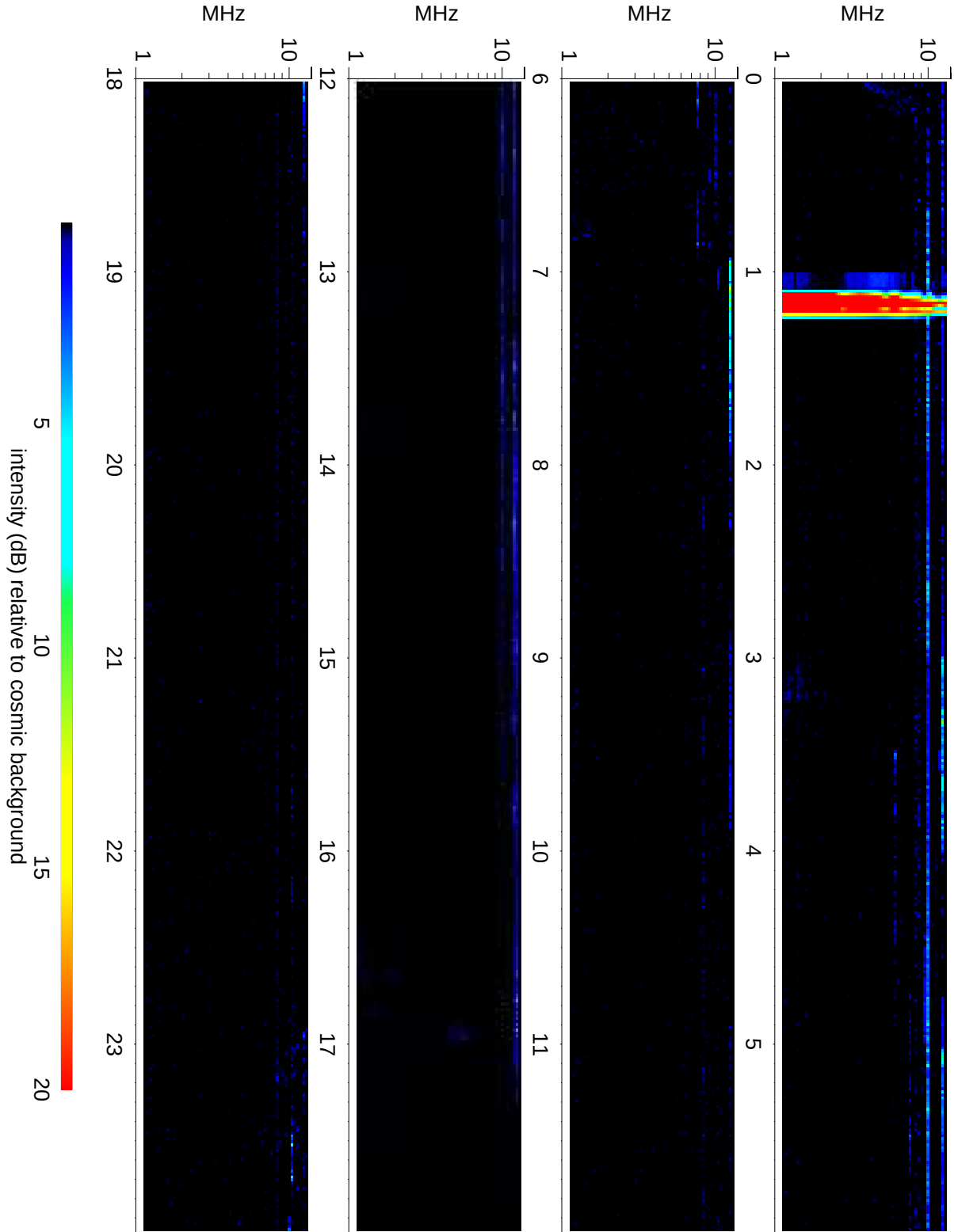
Wind Waves RAD2 receiver: 2020/05/05
