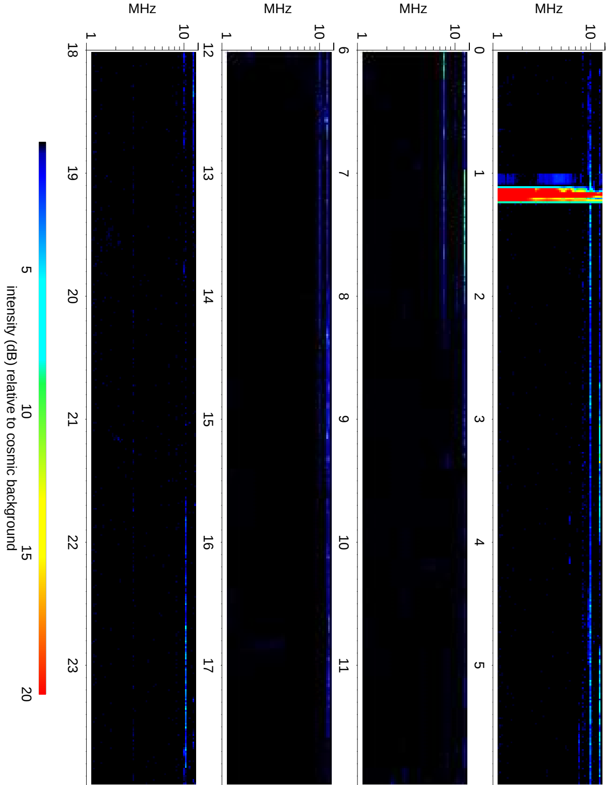
Wind Waves RAD2 receiver: 2020/05/09
