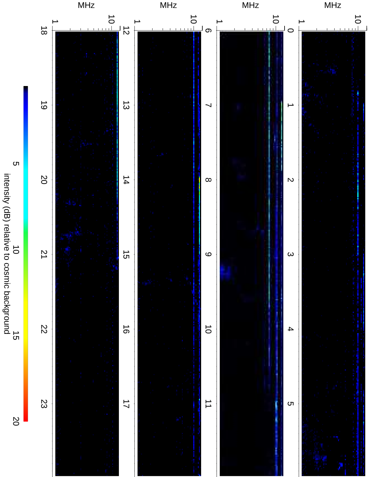
Wind Waves RAD2 receiver: 2020/07/09
