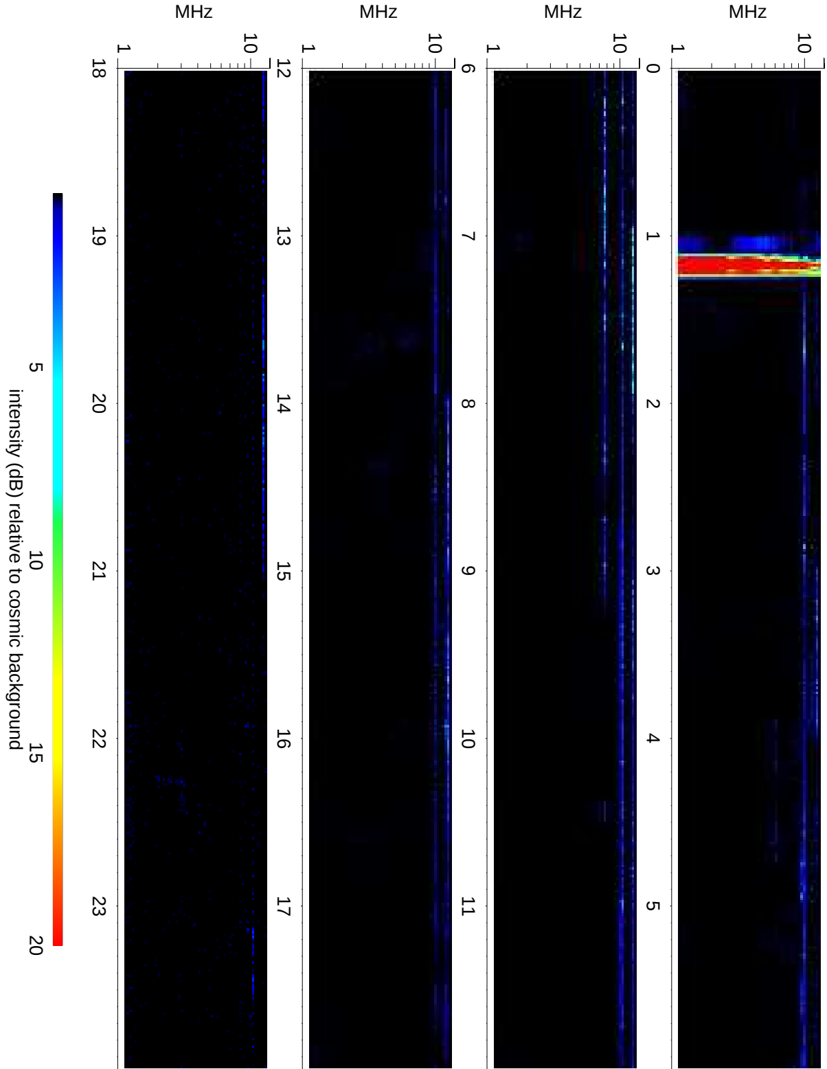
Wind Waves RAD2 receiver: 2020/07/24
