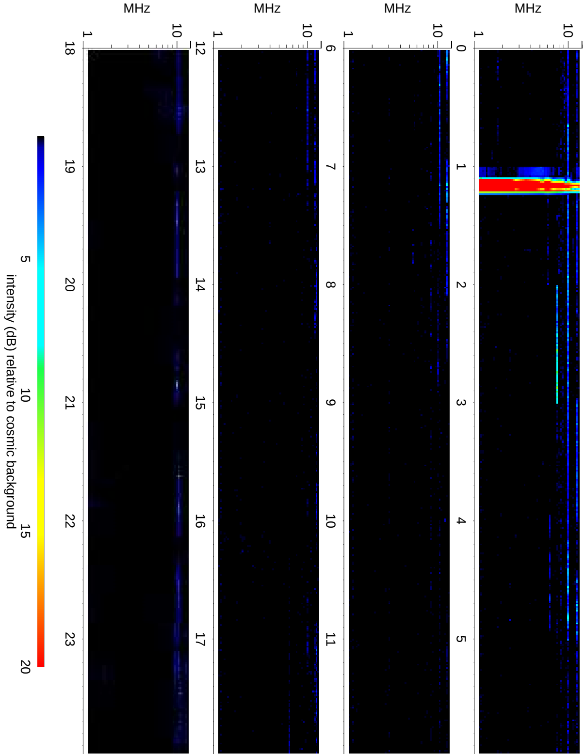
Wind Waves RAD2 receiver: 2020/09/28
