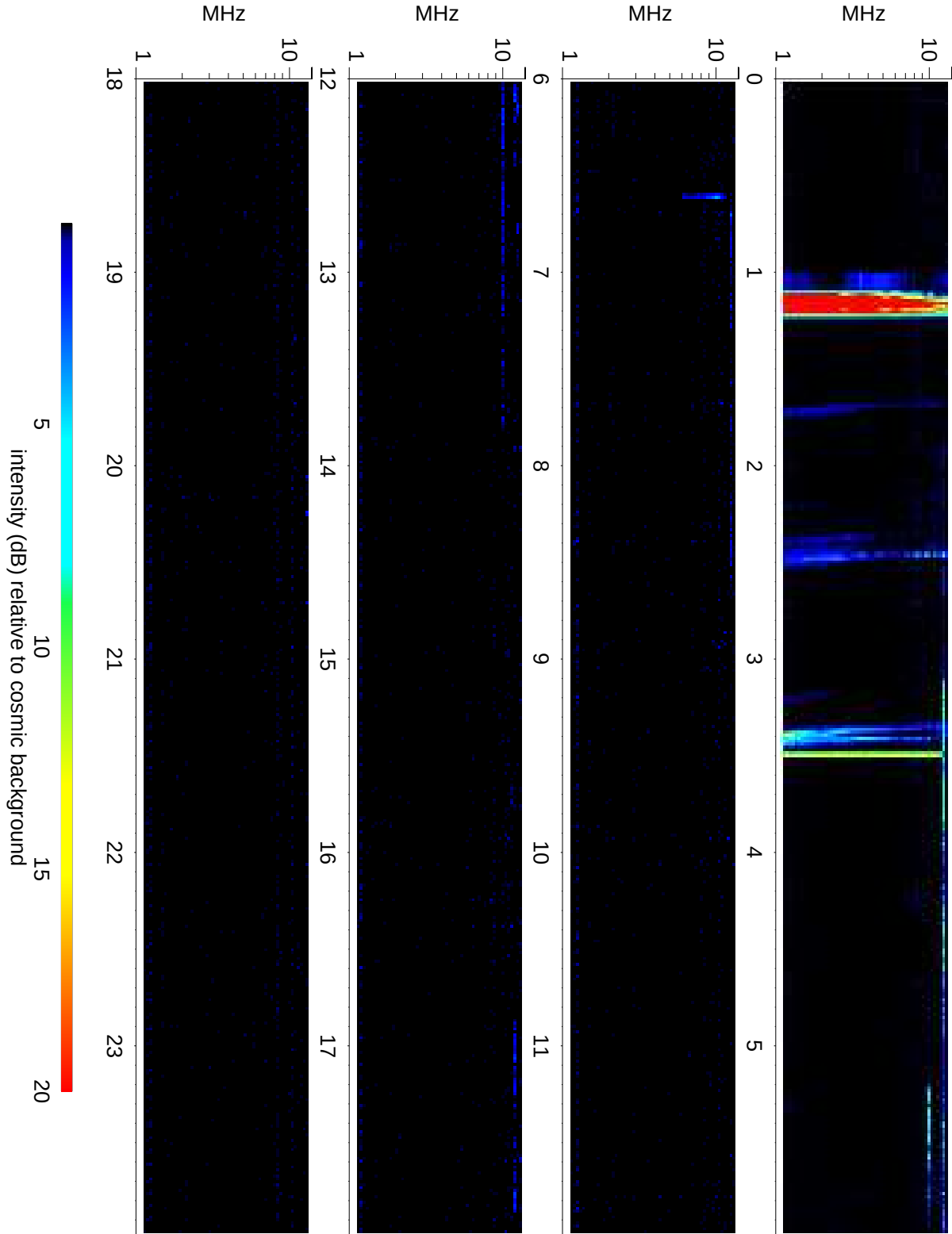
Wind Waves RAD2 receiver: 2020/11/13
