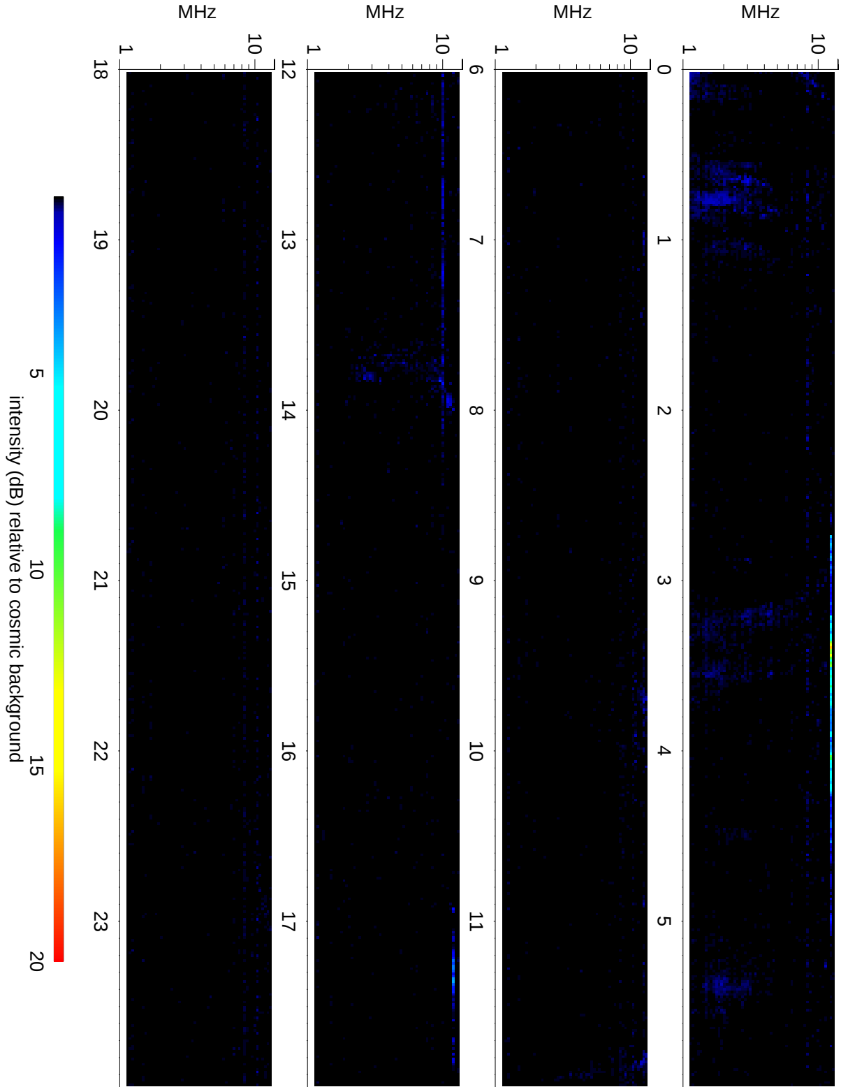
Wind Waves RAD2 receiver: 2020/11/16
