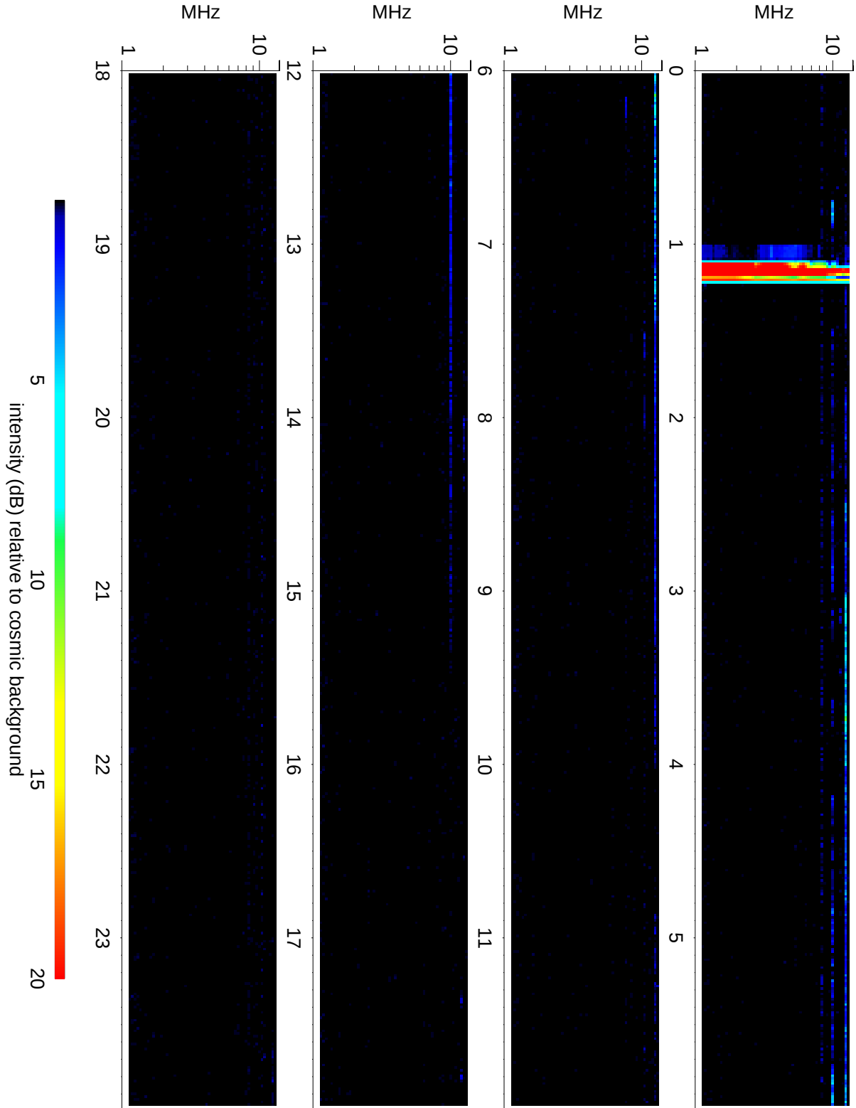
Wind Waves RAD2 receiver: 2021/01/30
