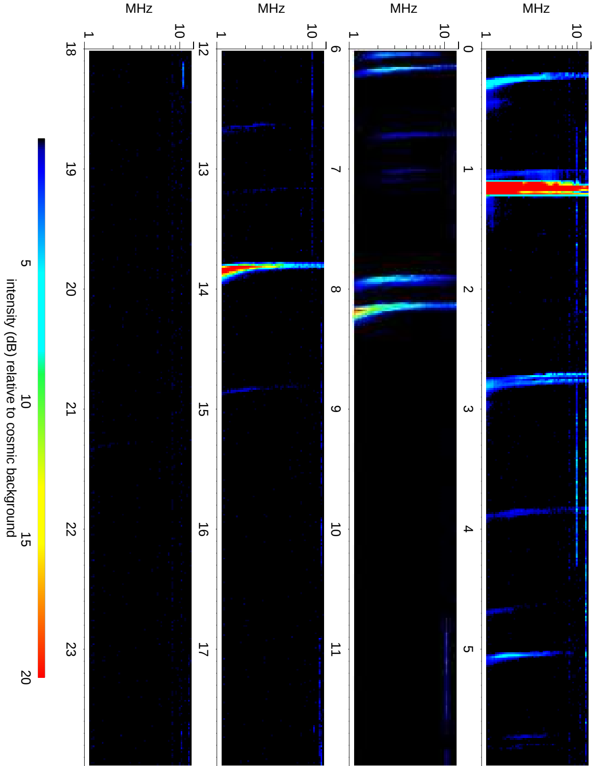
Wind Waves RAD2 receiver: 2021/03/01
