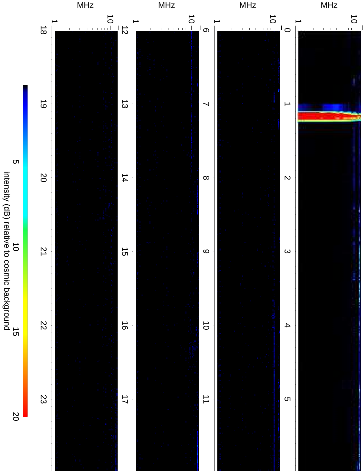
Wind Waves RAD2 receiver: 2021/03/15
