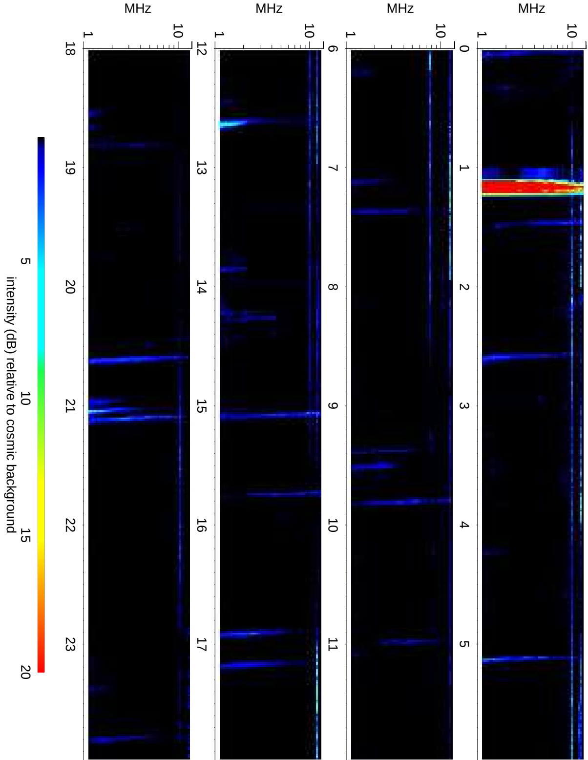
Wind Waves RAD2 receiver: 2021/05/08
