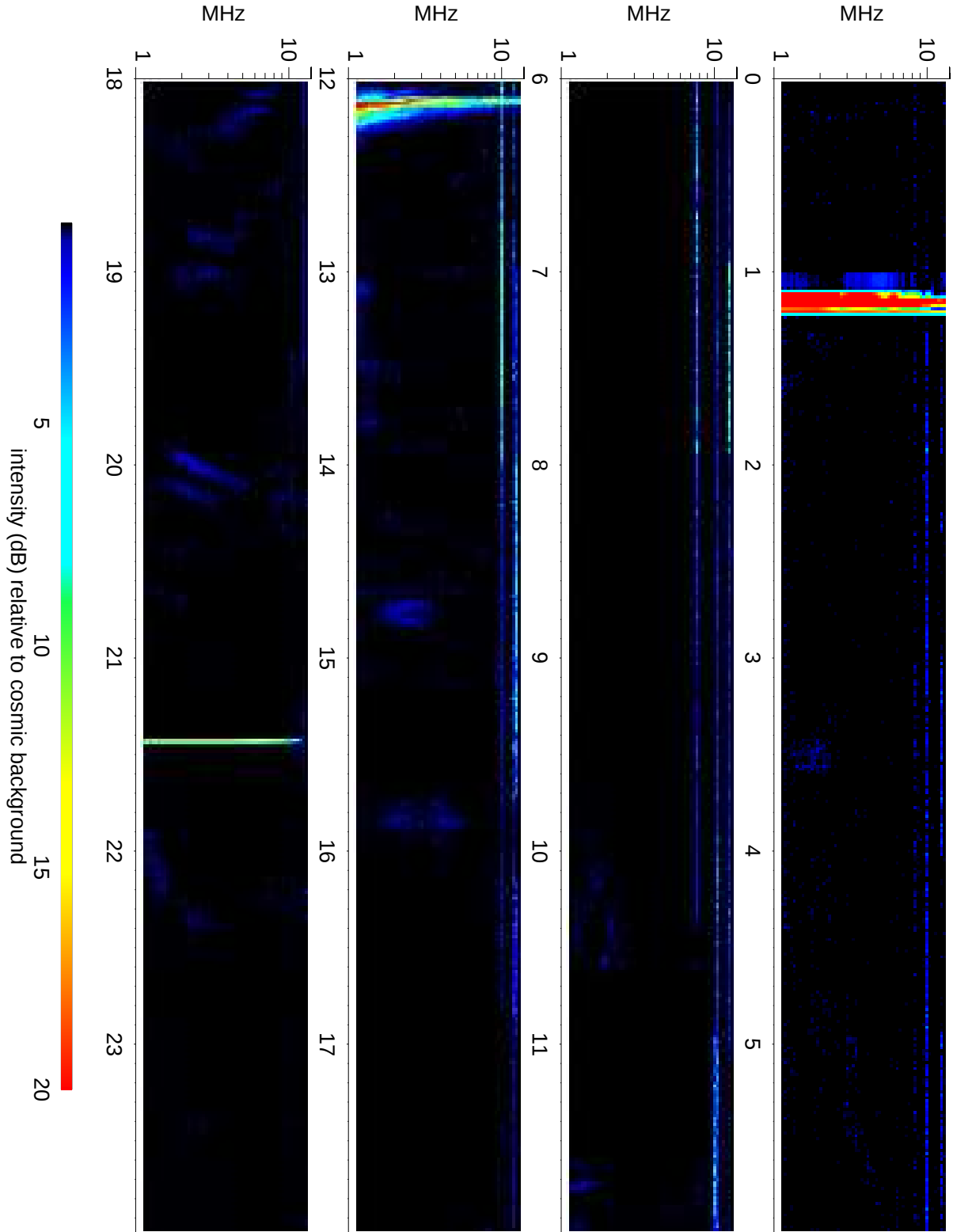
Wind Waves RAD2 receiver: 2021/06/09
