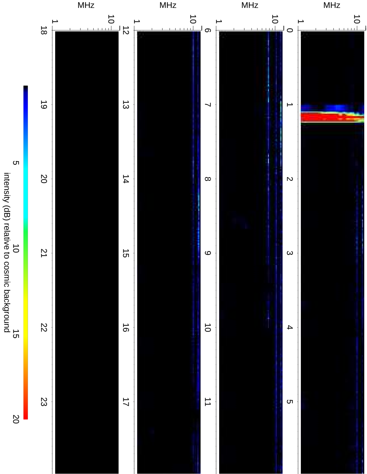
Wind Waves RAD2 receiver: 2021/07/07
