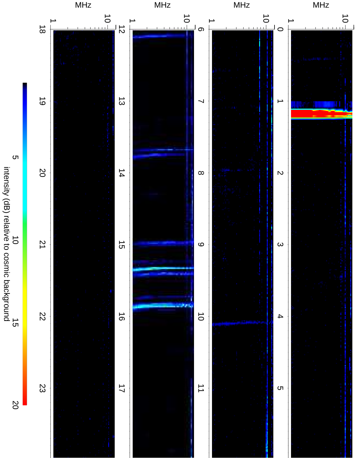
Wind Waves RAD2 receiver: 2021/07/19
