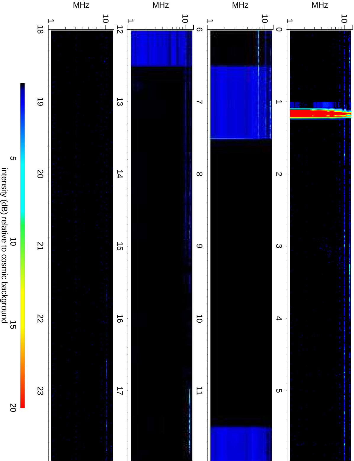
Wind Waves RAD2 receiver: 2021/08/08
