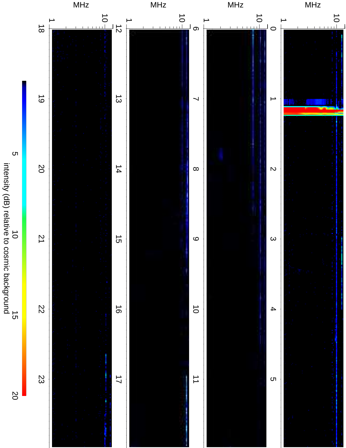
Wind Waves RAD2 receiver: 2021/08/12
