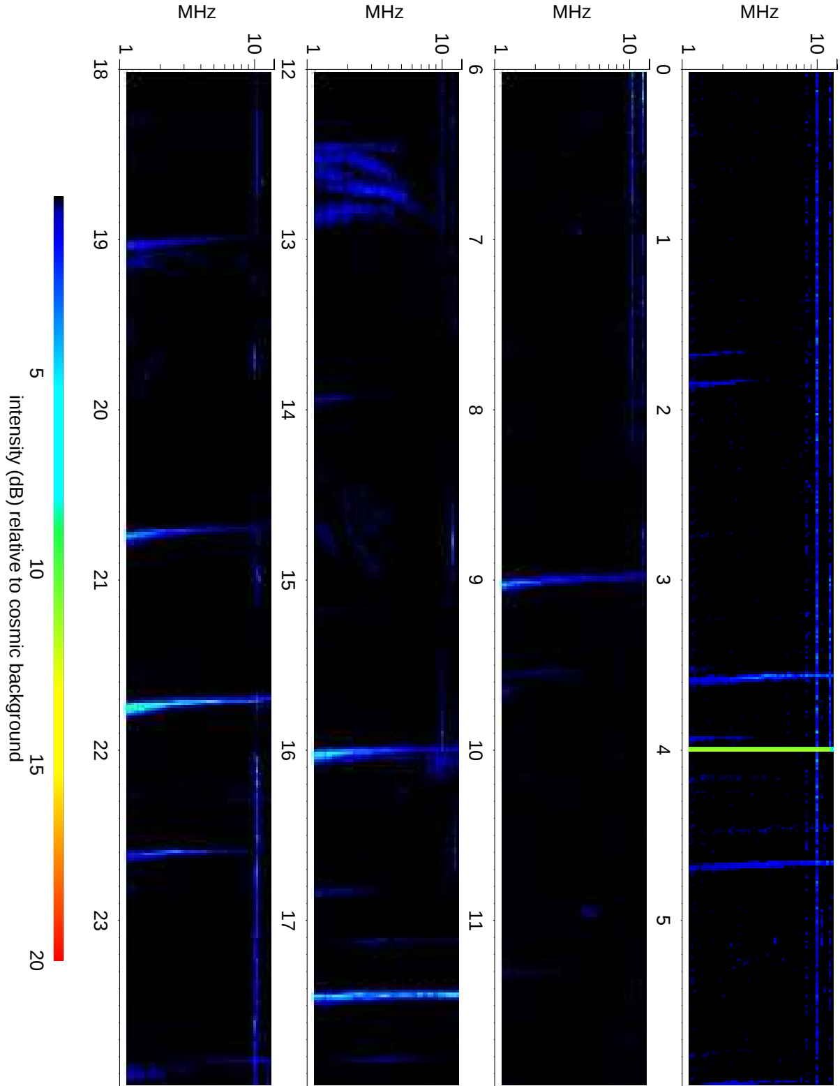
Wind Waves RAD2 receiver: 2021/09/20
