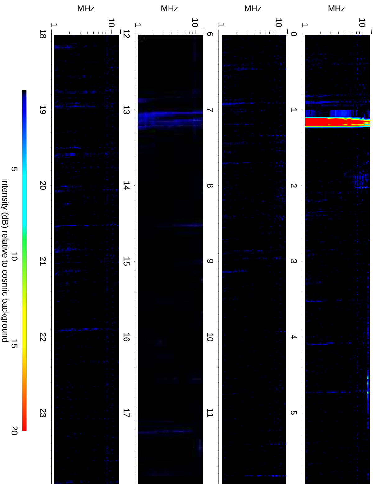
Wind Waves RAD2 receiver: 2021/11/08
