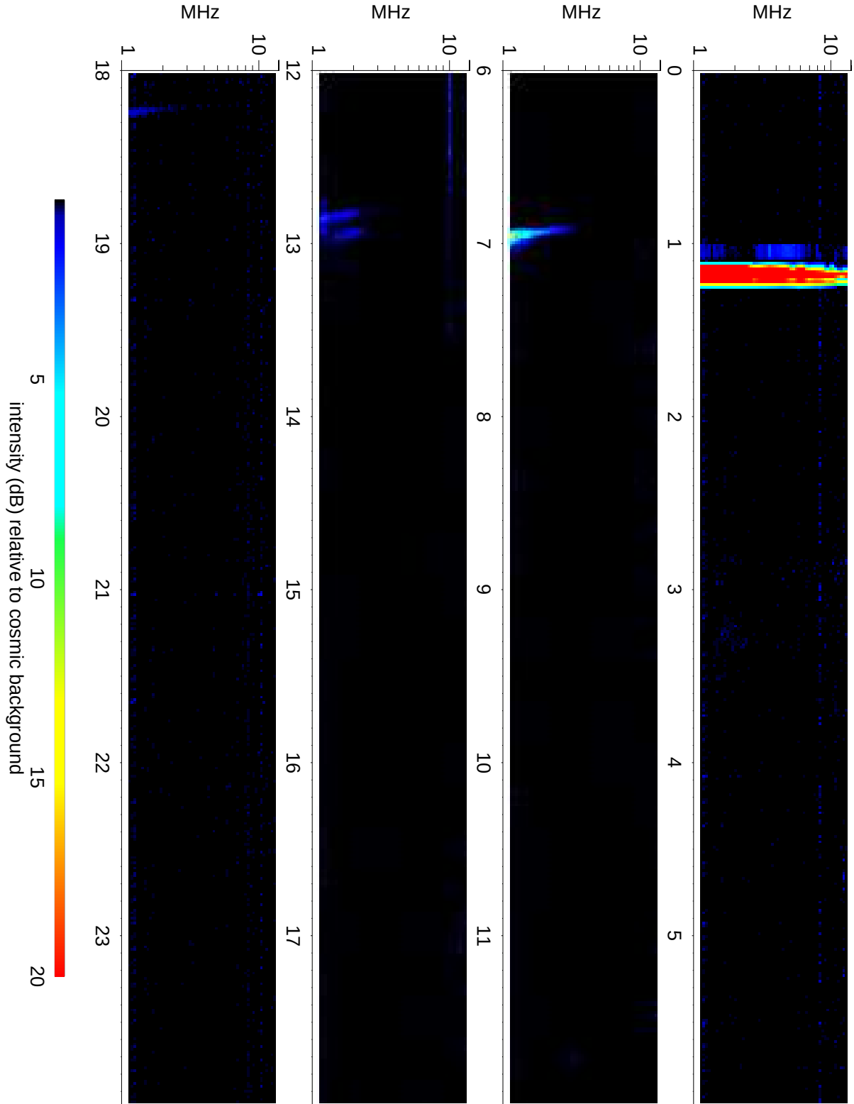
Wind Waves RAD2 receiver: 2021/11/18
