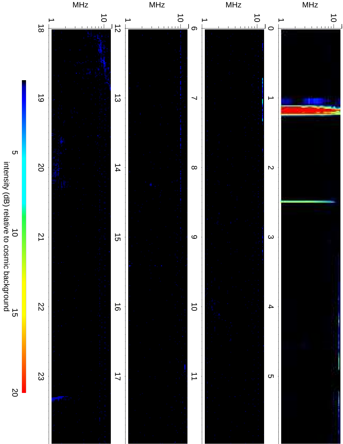
Wind Waves RAD2 receiver: 2021/11/26
