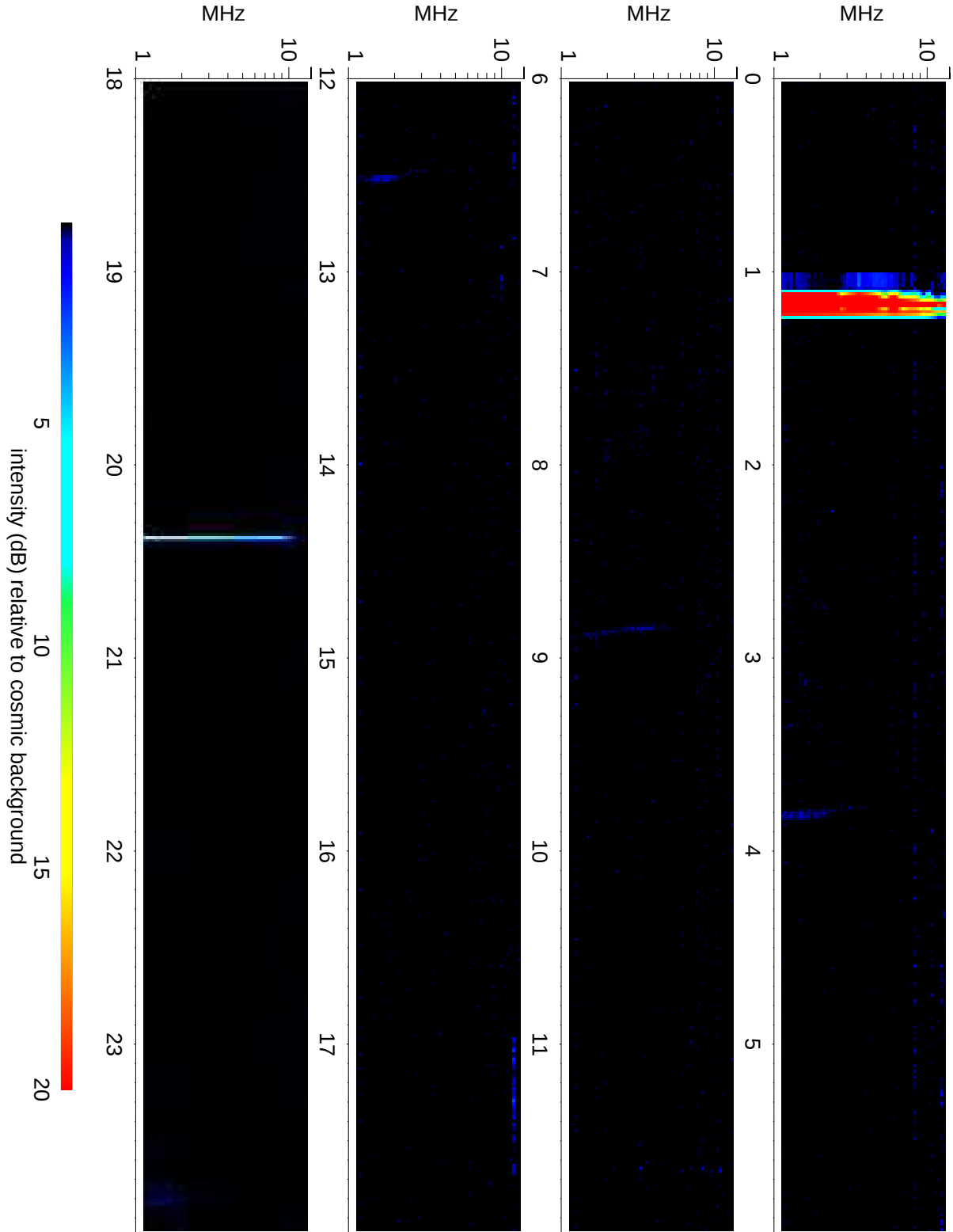
Wind Waves RAD2 receiver: 2021/11/30
